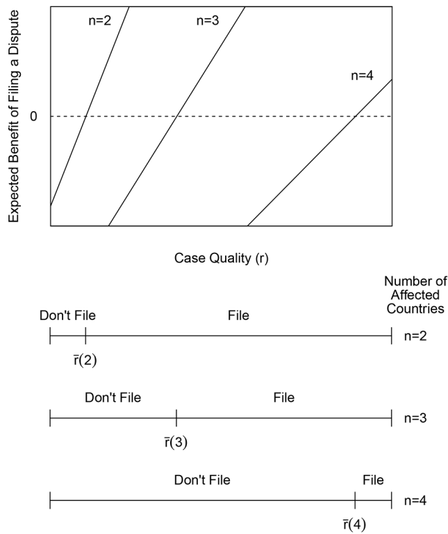
Figure 1. Diffuseness increases the quality of observed cases. Figure created from simulations of equilibrium behavior in R .
